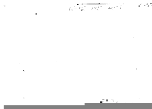
Fig. 5. A representative solid state ^{13}\text{C} NMR spectrum acquired from the isolated insoluble carbonaceous material (sample 120803-8).
